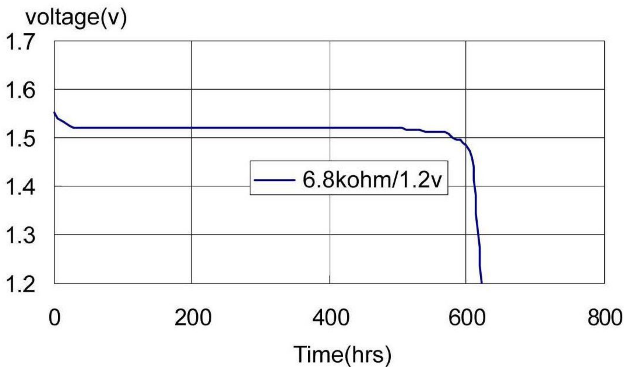
Typical Discharge curve at 20±2°C
